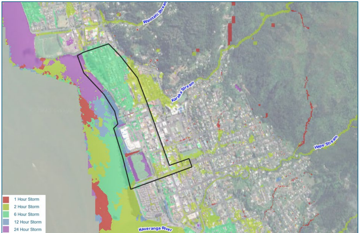
Figure 7-1: Critical Duration for Peak Water Level – 10 year ARI
