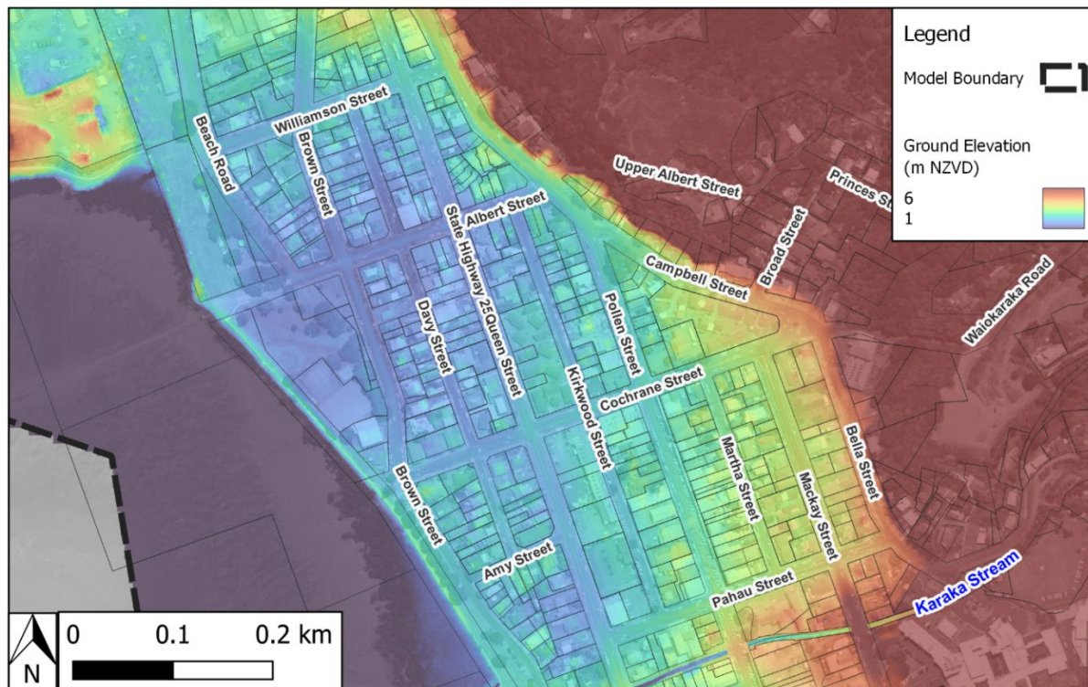
Figure 7-10: Ground Elevations in Thames
