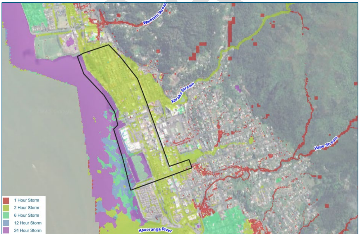
Figure 7-2: Critical Duration for Peak Water Level – 50 year ARI
