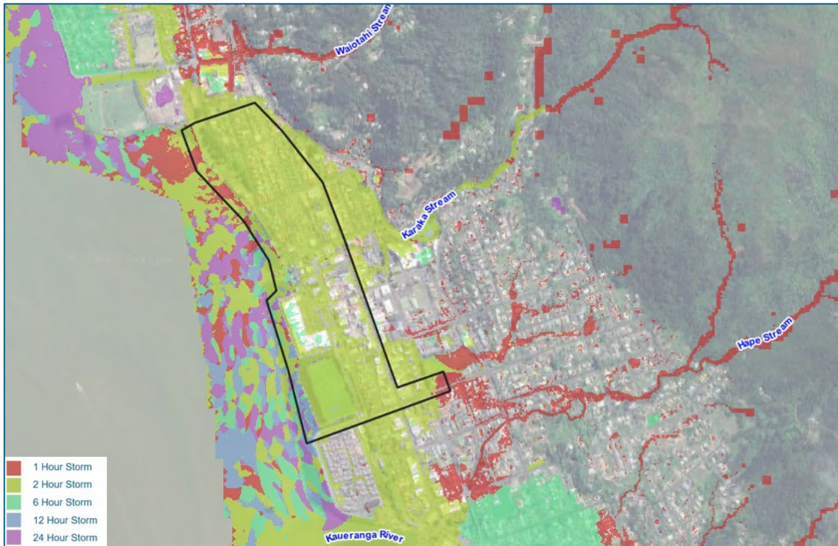
Figure 7-3: Critical Duration for Peak Water Level – 100 year ARI
