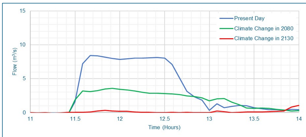
Figure 7-13: Flow in Karaka Stream at the Brown Street Bridge – 100 year ARI Event
