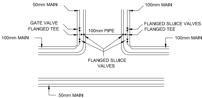
TEE INTERSECTION 2
