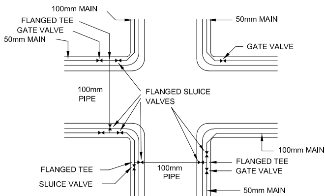
CROSS INTERSECTION
