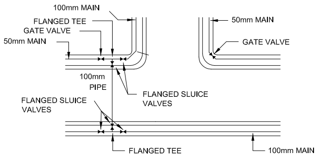
TEE INTERSECTION 1
