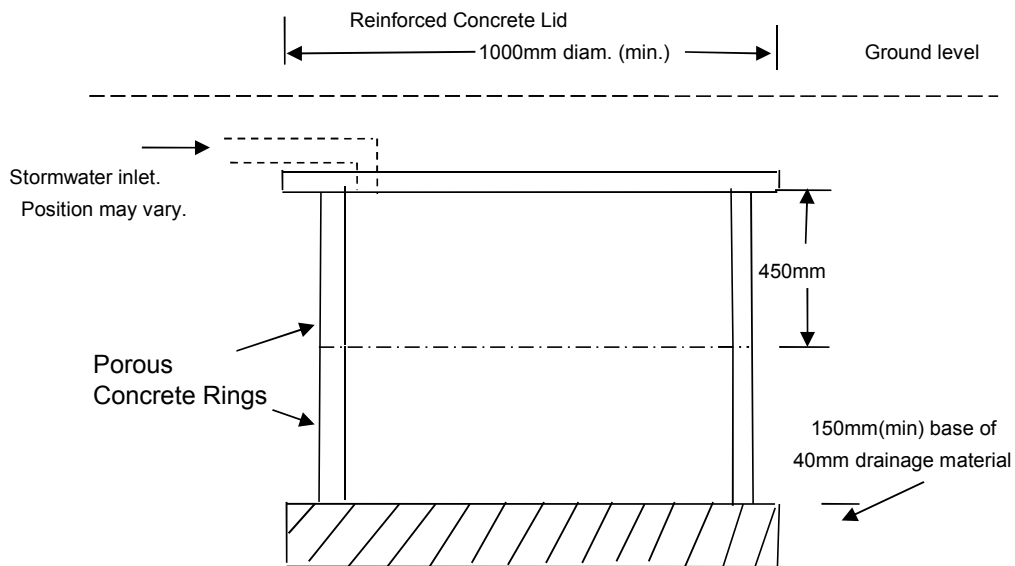
Section: Typical on-site stormwater retention well. Showing two standard 900mm diam. porous concrete rings.
