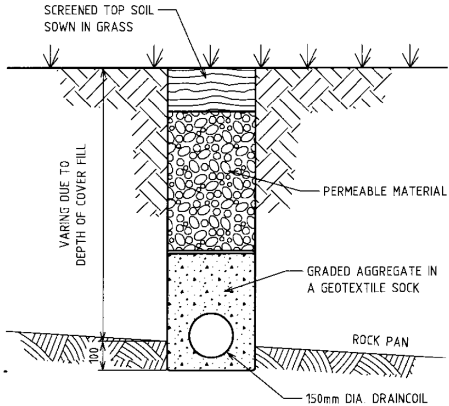
TYPICAL SUBSOIL DRAIN TO CUT OFF UNDERGROUND WATER FLOW FOLLOWING GRADIENT OF ROCK PAN.
